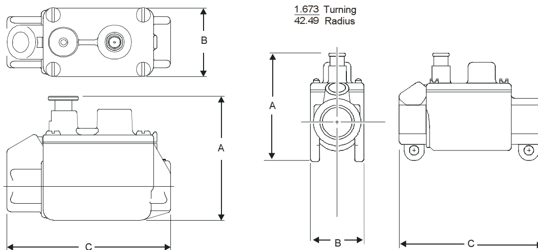
H17 Dimensions
