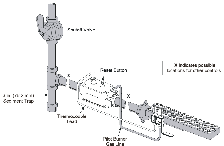
Typical H17 Installation
