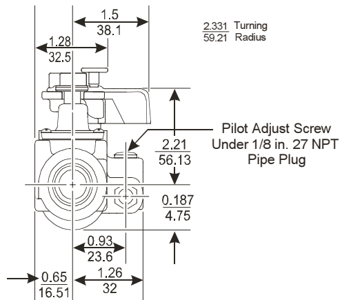
H43 Dimensions (in./mm)
