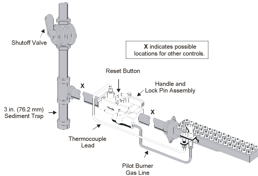
Typical H43 Installation
